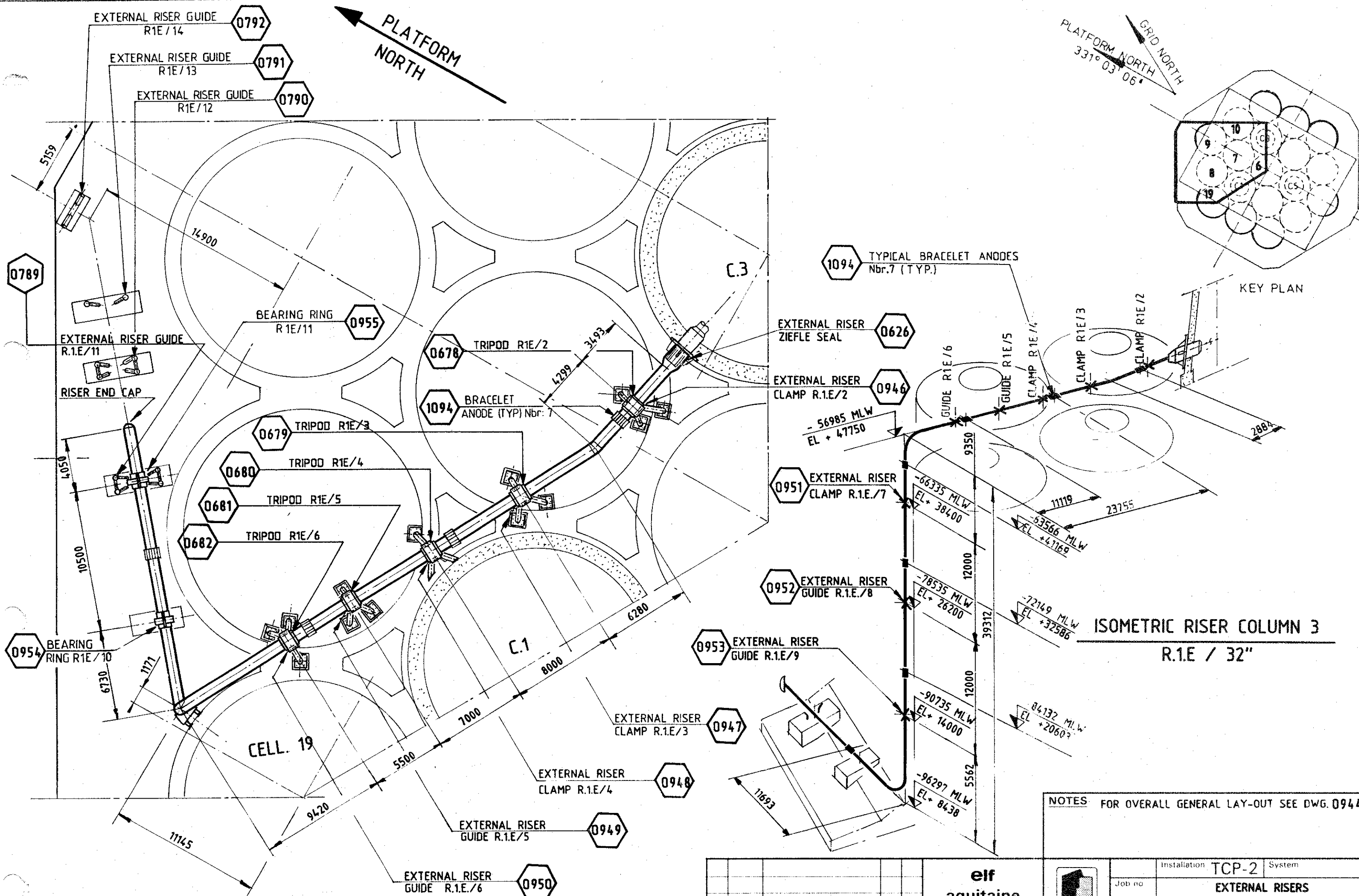
PLAN VIEW Scale 1/250
