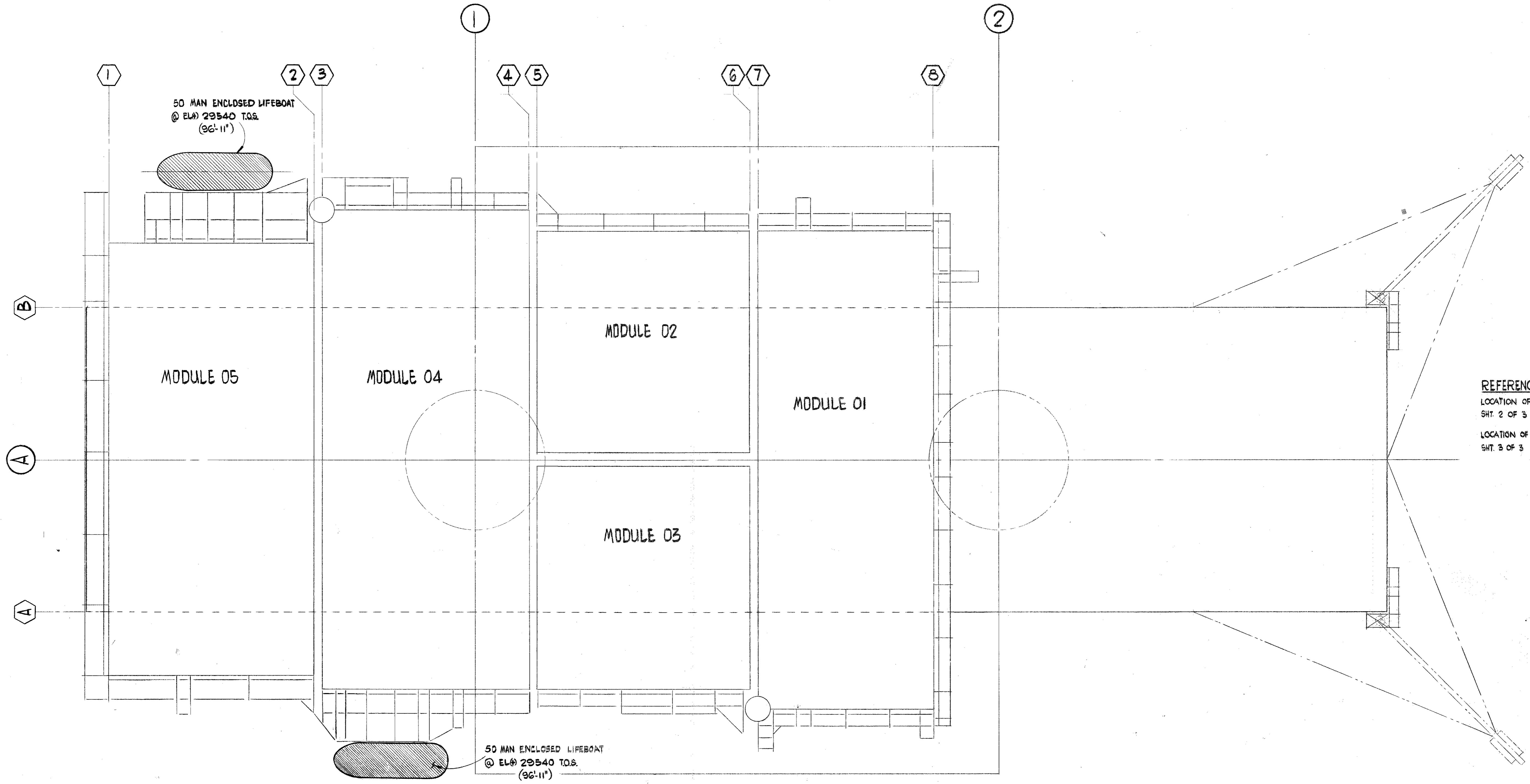
PLAN ON T.P.I. SHOWING LOCATION OF LIFEBOATS SCALE 1:150
