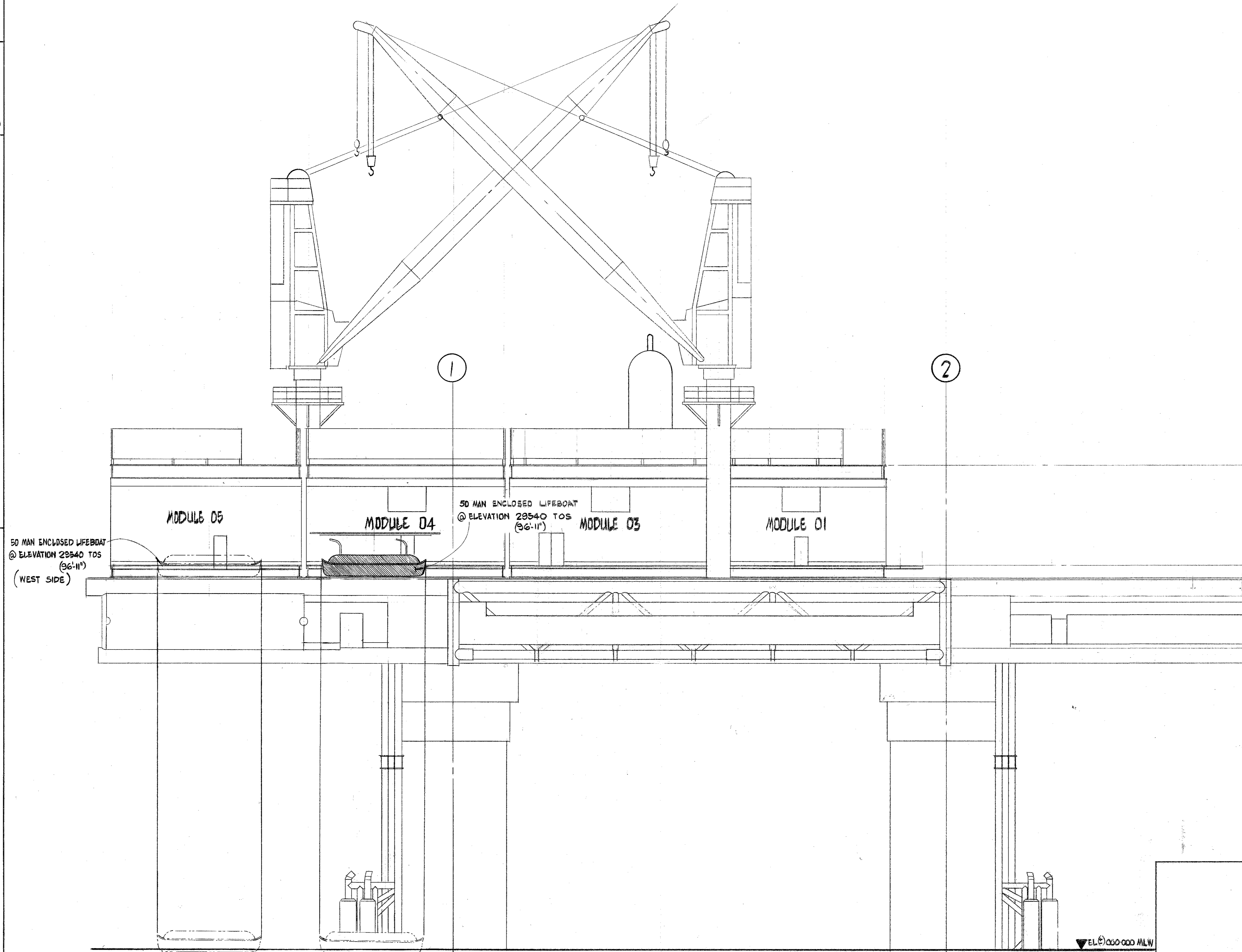
EAST ELEVATION ON TPI SHOWING LOCATION OF LIFEBOATS SCALE 1:150.
