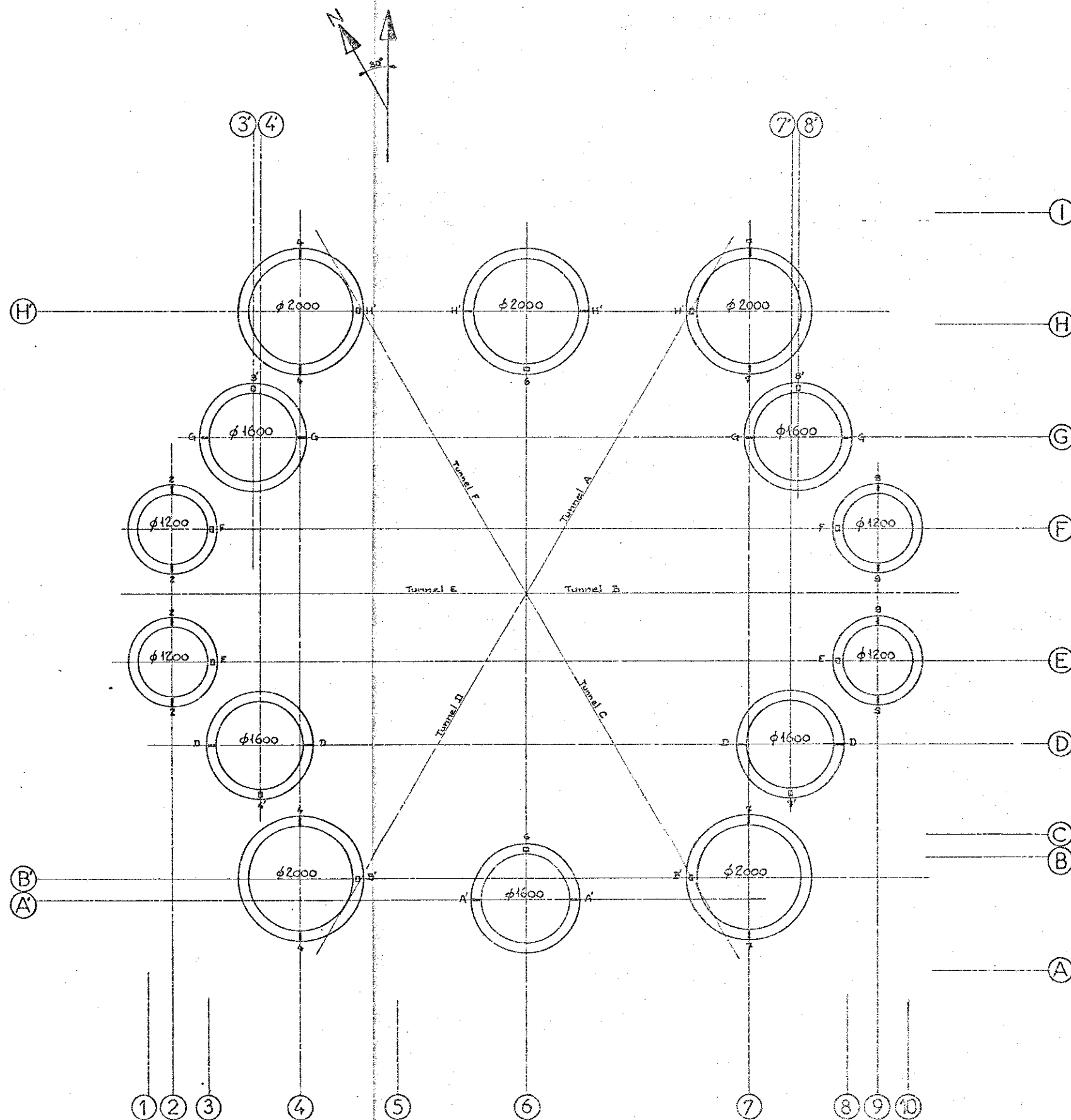
GENERAL LAYOUT
