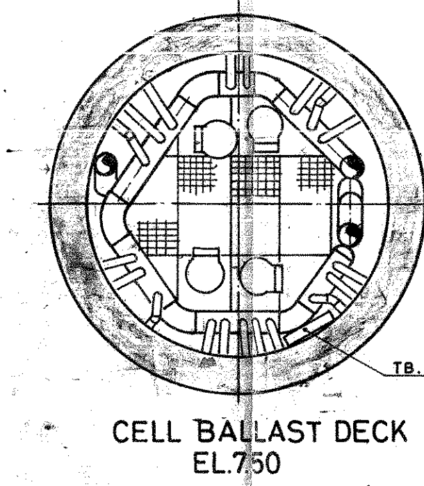
DECK DETAILS SCALE 1:100
