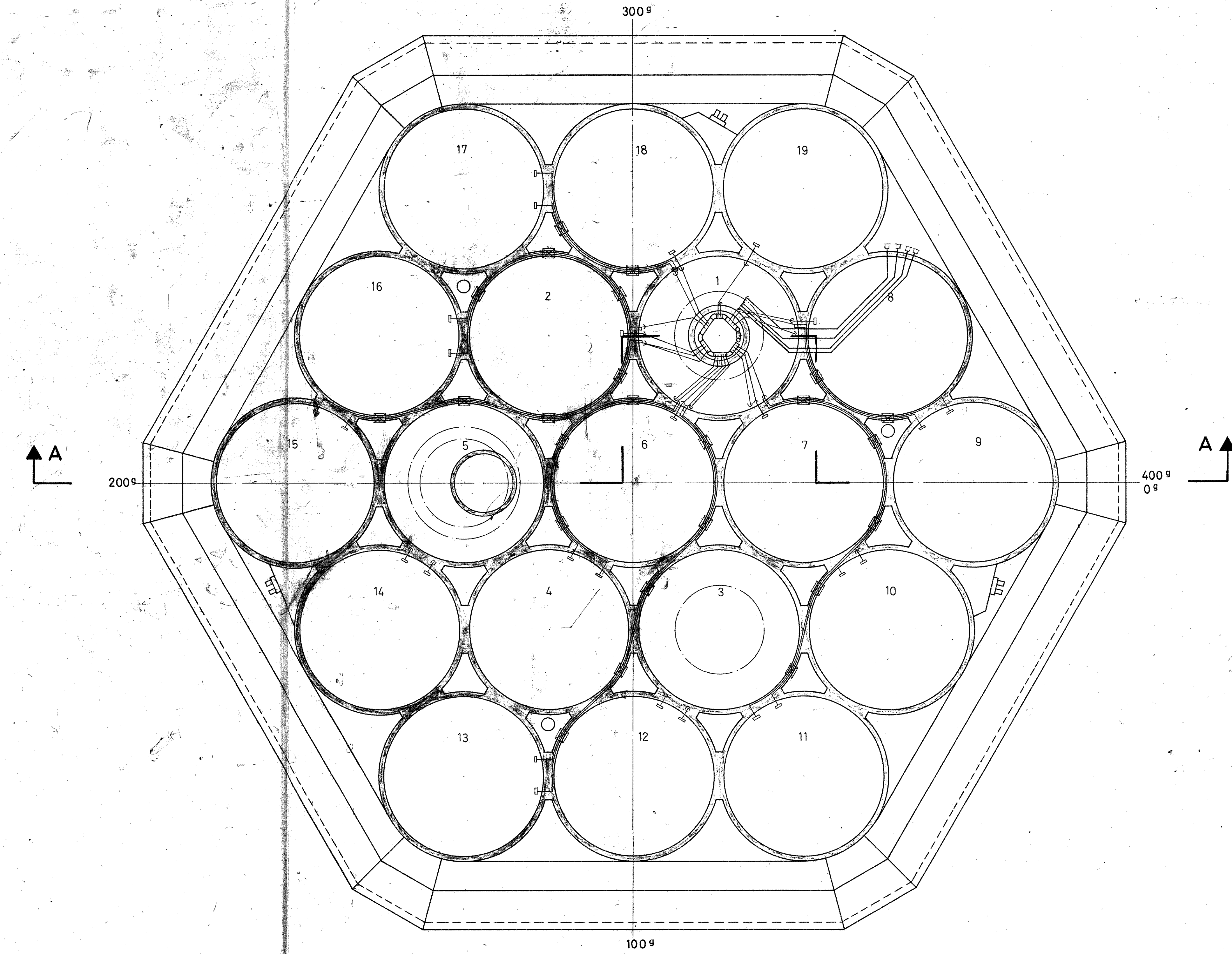
DECK DETAILS SCALE 1:100
