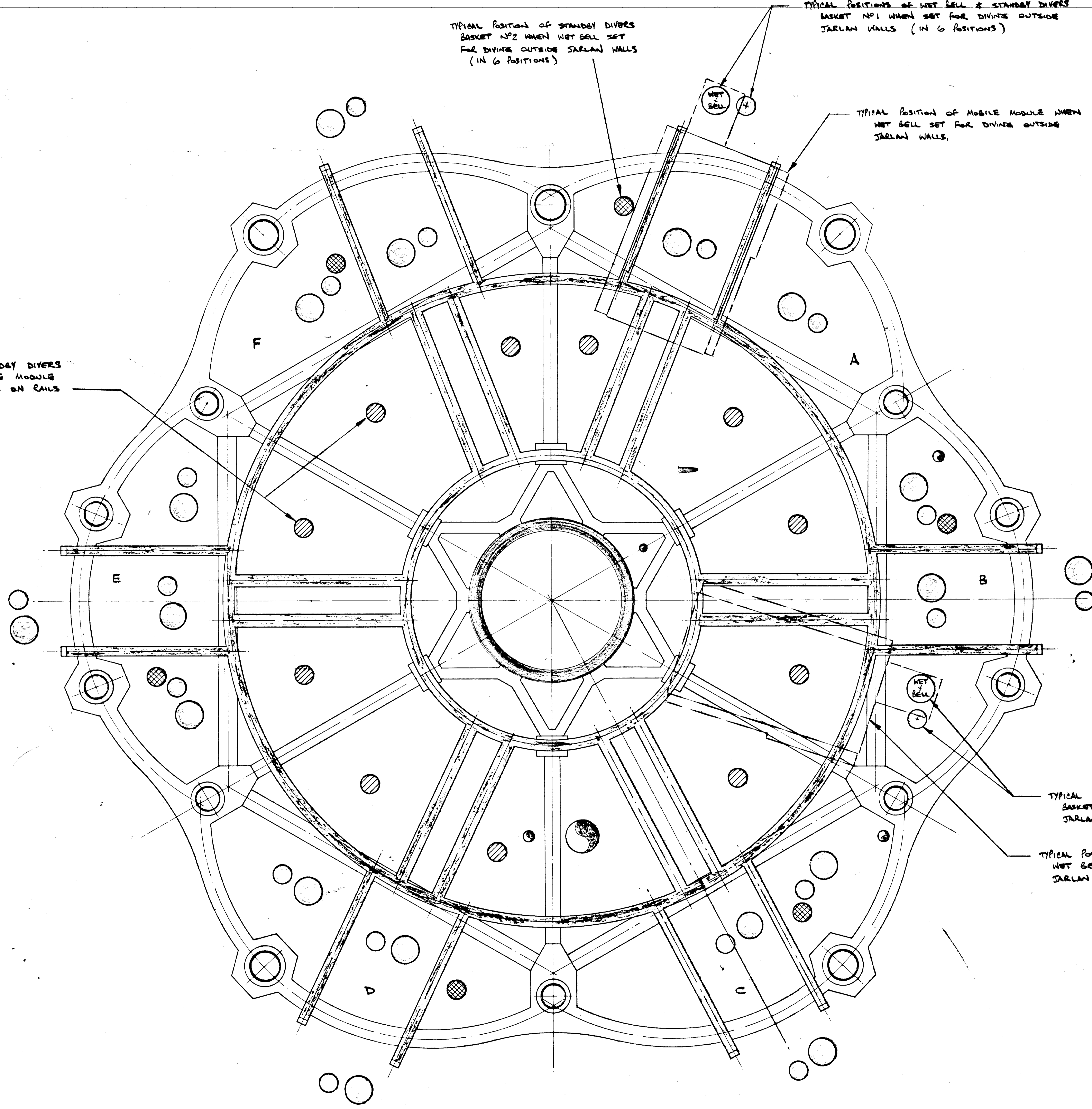
PLAN VIEW AT EL 108,000
