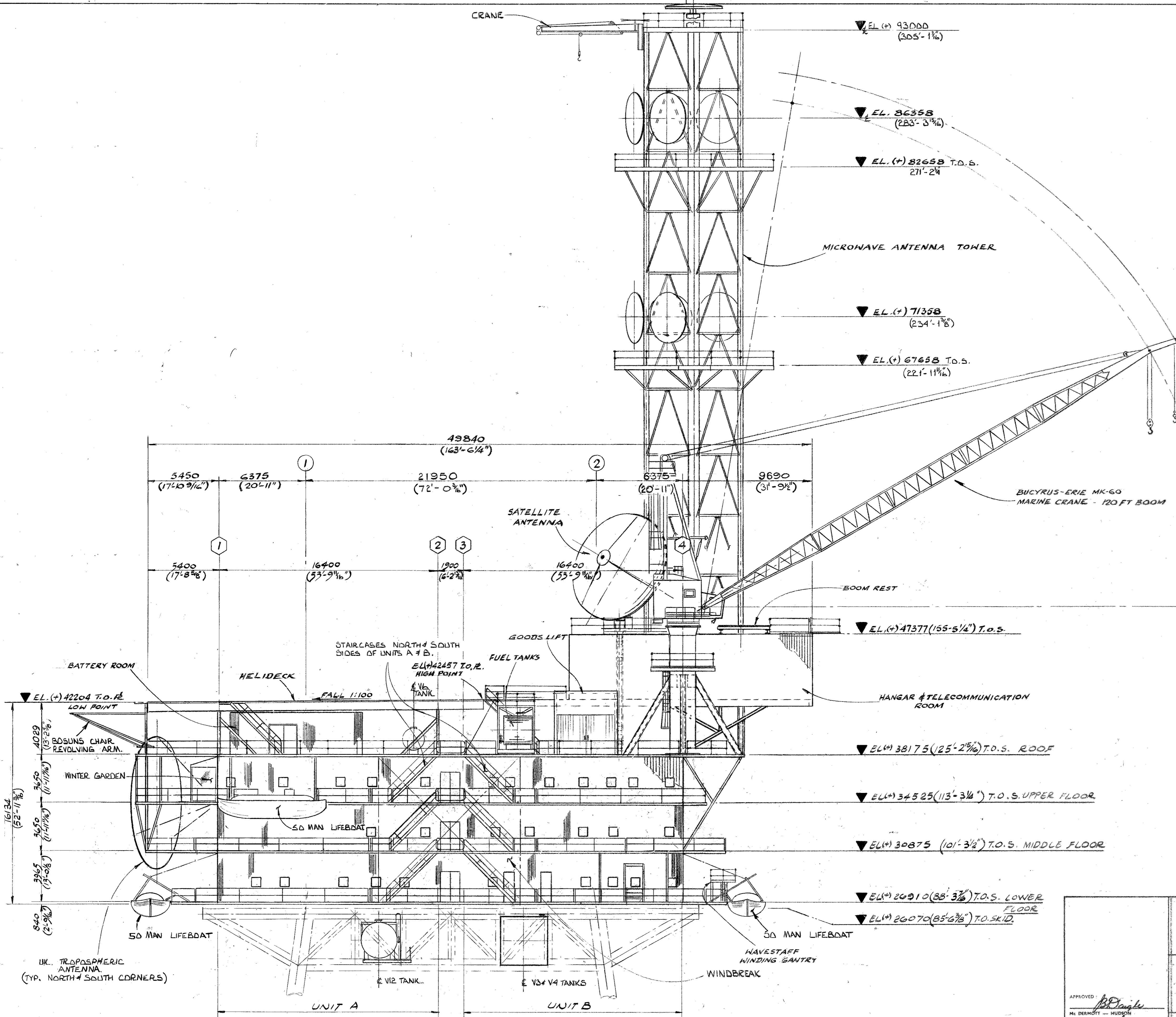
SOUTH ELEVATION (WINDSCREEN REMOVED FOR CLARITY)
